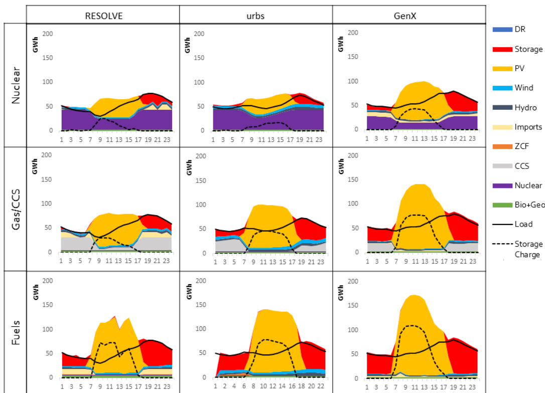
Figure 6. Each type of clean firm power would play a slightly different role in meeting demand. Daily generation pattern of the three models on an example September day for each scenario. Nuclear power would act as a “flexible base” power source but conserving fuel by reducing output during the height of solar output. Natural gas generation with CO 2 capture and storage would ramp up at night when solar ramps down. Use of costly carbon-free fuels would only run when solar, wind and storage options were unavailable. Any of these resources could fill the gap during times of dunkelflaute . Each clean firm resource shows distinct daily operations that are consistent across all three models. Note: Representative September day used for RESOLVE, average generation profile for September days used for urbs, and average generation profile of representative September weeks used for GenX. GenX imports indicate net imports into California, and may include imports of power from clean firm resources operating outside of California. (Figure taken from Baik et al. “What is different about different net-zero carbon electricity systems?”, manuscript EGYCC-D-20-00141 (under review) in Energy and Climate Change ).
