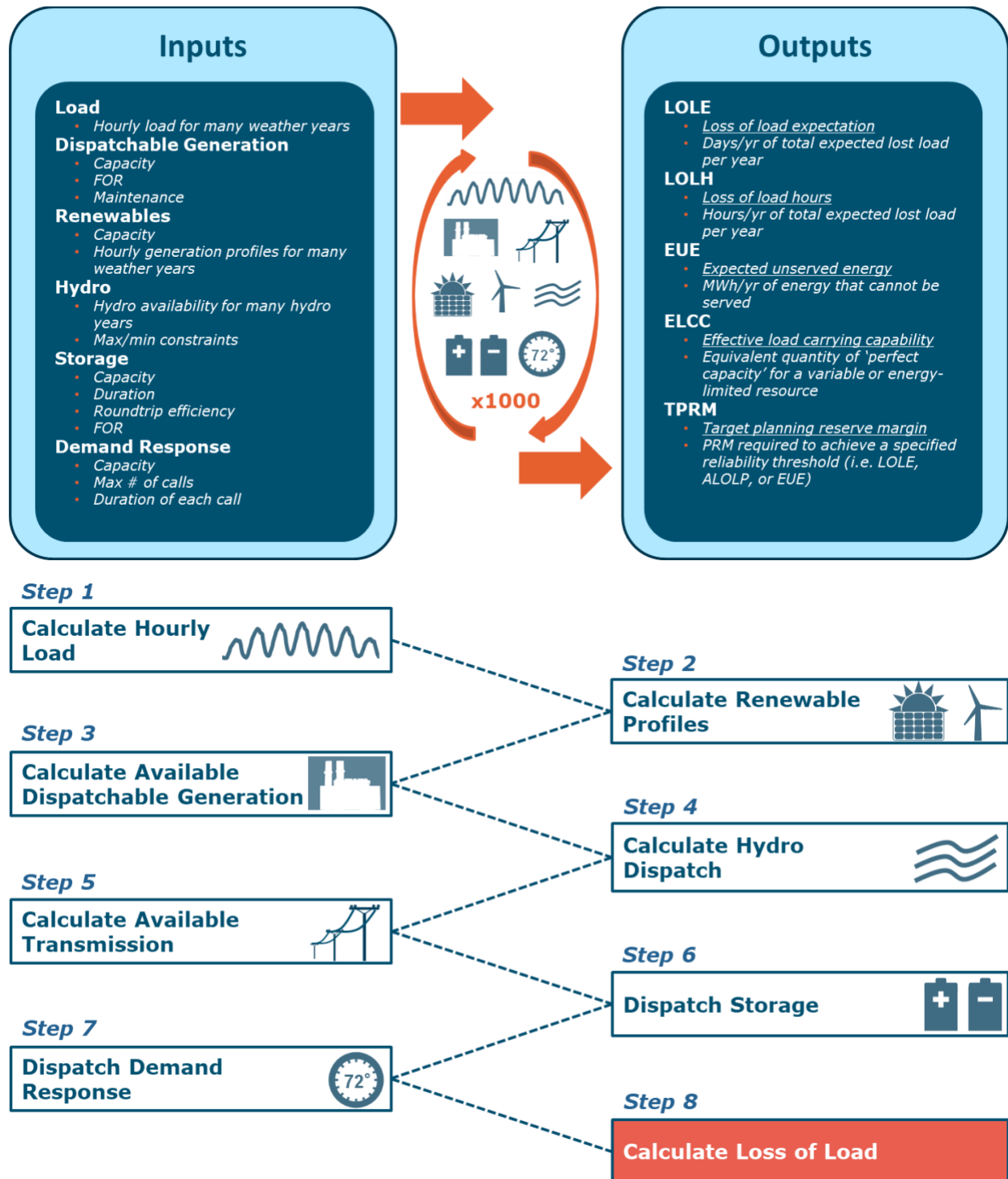
Figure 2. Overview of RECAP model
