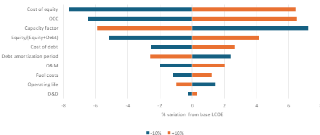
Figure 6. Sensitivity Analysis of input parameters on LCOE.
