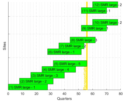
Figure 18. Deployment schedule assumed for the high trend.
