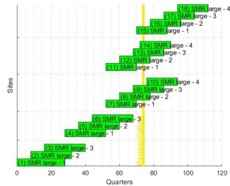
Figure 12. Deployment schedule assumed for the high trend (SMR as new capacity).
