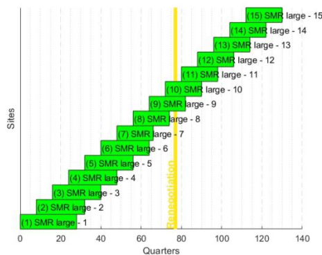
Figure 13. Deployment schedule assumed for the low trend (SMR as replacement).
