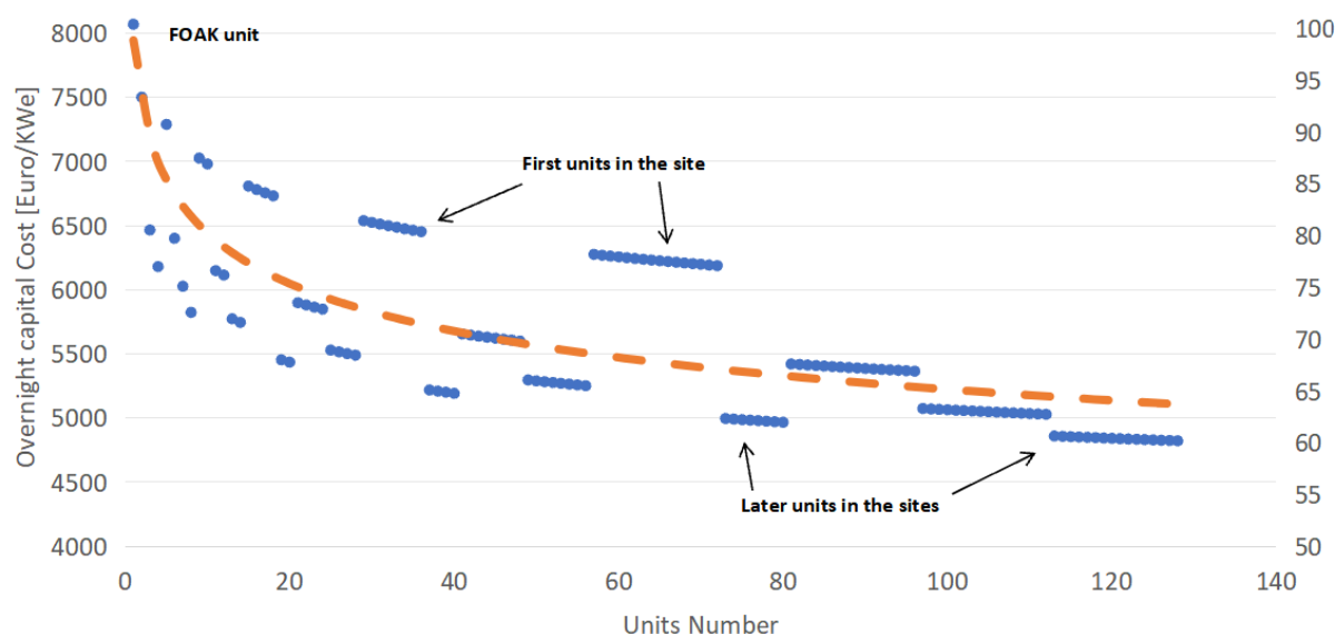
Figure 5. Single unit capital cost by build sequence (51.2 GWe fleet, 32 sites of 1600 MWe, 4x400 MWe units per site, optimistic assumptions)
