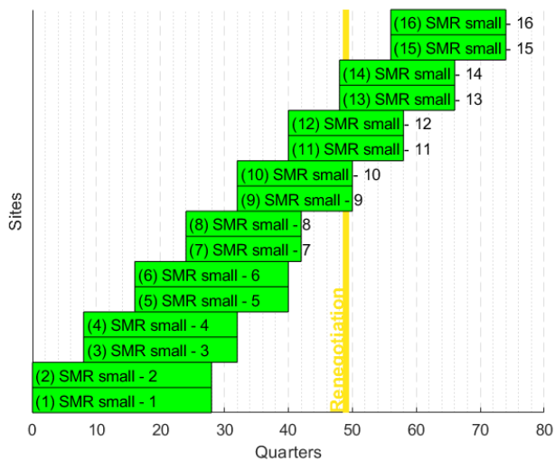
Figure 10. Example of deployment schedule: C3 scenario with 100 MWe units (16x100 MWe example).
