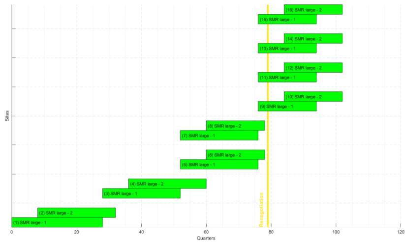
Figure 10. Example of deployment schedule: C3 scenario with 100 MWe units (16x100 MWe example).
