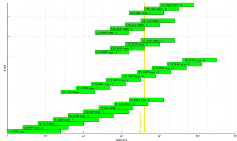
Figure 24. Deployment schedule assumed for the high trend (SMR as replacement).
