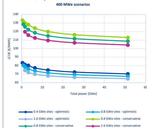
Figure 2. LCOE variation against total deployed capacity: 400 MWe reactor-unit scenarios, optimistic and conservative.
