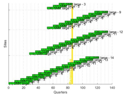
Figure 14. Deployment schedule assumed for the medium trend (SMR as replacement).
