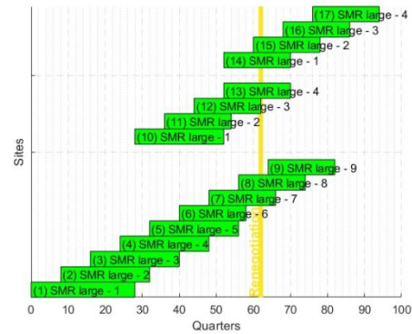
Figure 24. Deployment schedule assumed for the high trend (SMR as replacement).
