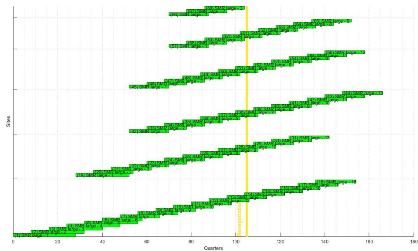
Figure 15. Deployment schedule assumed for the high trend (SMR as replacement).
