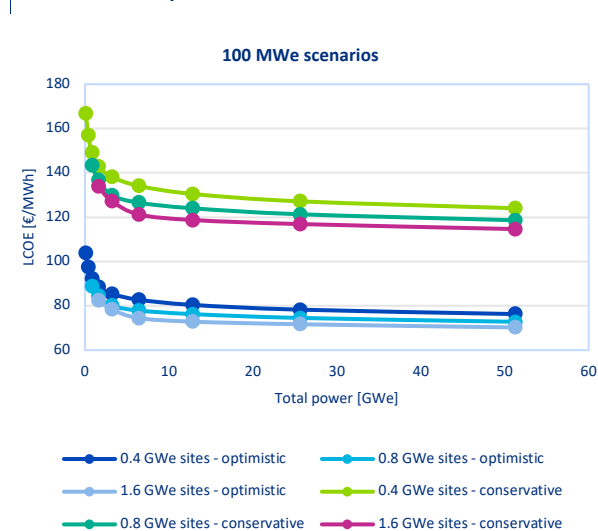
Figure 3. LCOE variation against total deployed capacity: 100 MWe reactor-unit scenarios, optimistic and conservative.
