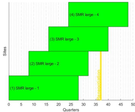
Figure 19. Deployment schedule assumed for the low trend (SMR as new capacity).
