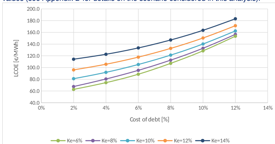
Figure 7. Financing leverage: LCOE variation under varying cost of debt and cost of equity values (see Appendix D for details on the scenario considered in this analysis).
